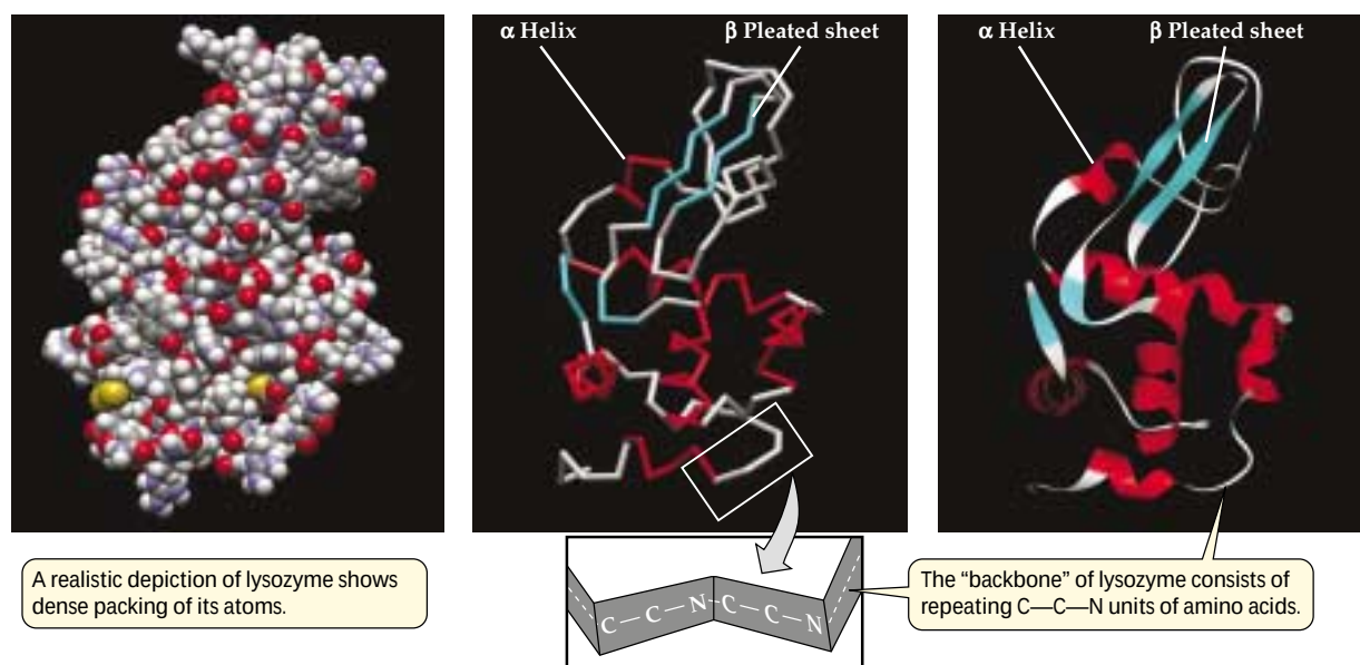
3.7 Three Representations of Lysozyme Different molecular representations of a protein emphasize different aspects of its tertiary structure. These three representations of lysozyme are similarly oriented.
