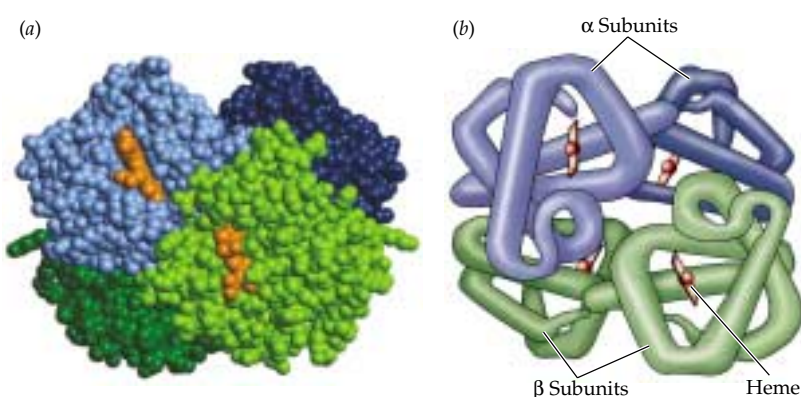
3.8 Quaternary Structure of a Protein Hemoglobin consists of four folded polypeptide subunits that assemble themselves into the quaternary structure shown here. In these two graphic representations, each type of subunit is a different color. The heme groups contain iron and are the oxygen-carrying sites.
