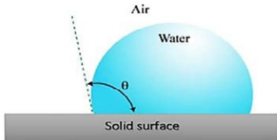
A Hydrophobic System Based on Silicon Oxide (SiO 2 ) Coated Surface.
