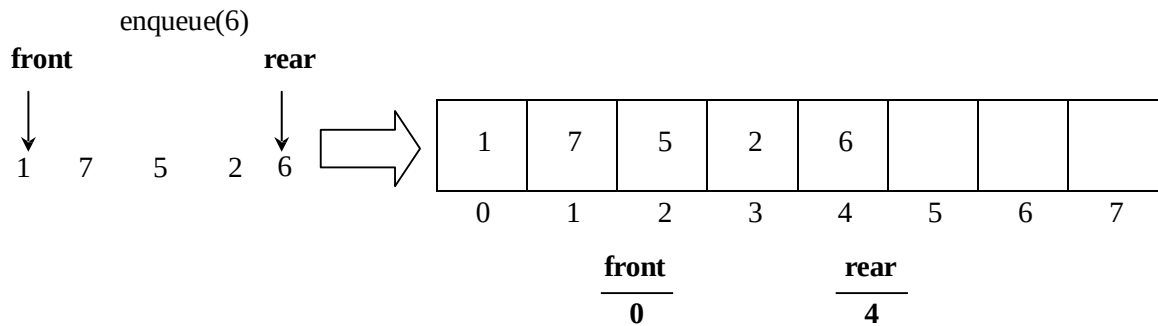
Fig 7. Insertion of one element 6
