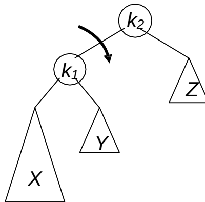
Fig 23.1: Single Right Rotation
