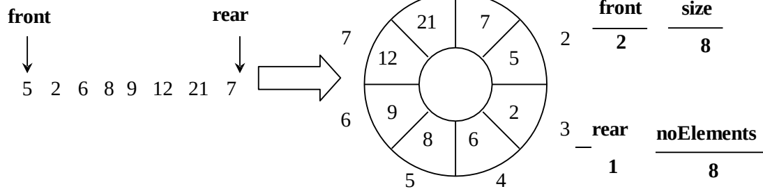
Fig 14. Another element added in circular array
