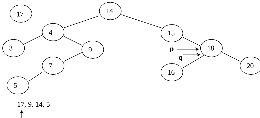
Fig 12.12: Insertion of a new node in progress
