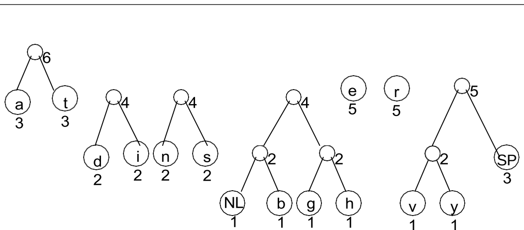
Fig 26.4: joining different nodes to create new nodes
