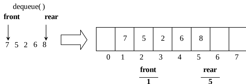
Fig 9. Removal of an element from front
