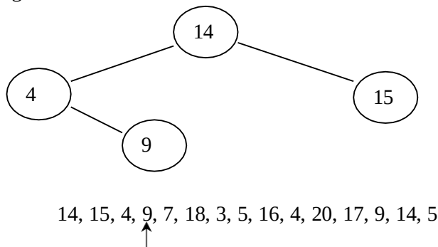
Fig 12.7: A new node is added in the tree
