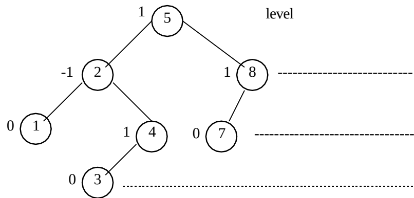
Fig 20.2: balance of nodes in an AVL
