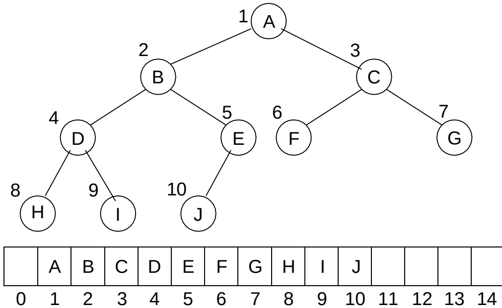
Figure 29.1: Complete Binary Tree
