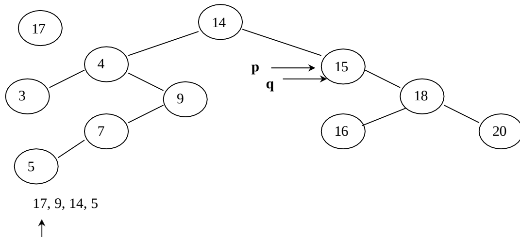
Fig 12.11: Insertion of a new node in progress
