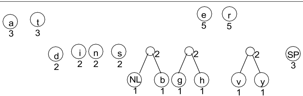
Fig 26.3: joining leaf nodes to create new nodes
