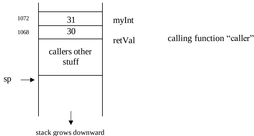
Fig 17.5 call stack layout after return from intMinus1
