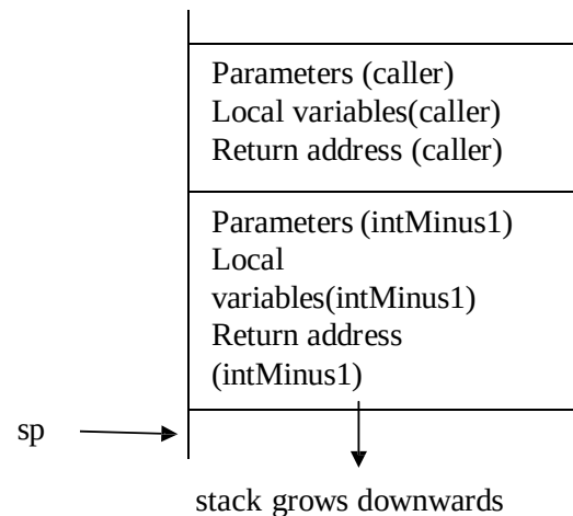
Fig 17.2: call stack layout
